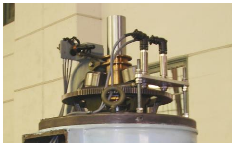
Figure 1. Modified PMG for Digital Speed Sensing
