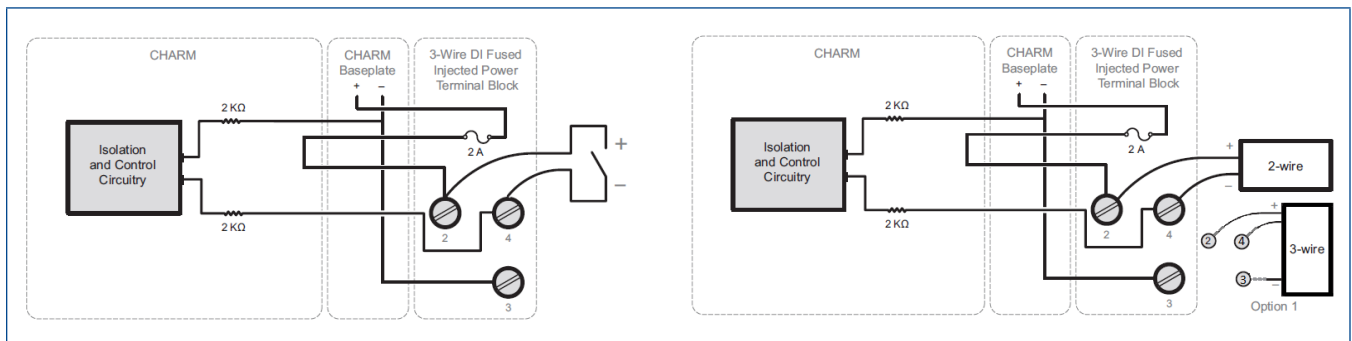
Simplified Circuit and Connection Diagrams for DI 24 V DC Isolated CHARM with 3-wire DI Fused Injected-Power Terminal Block.
