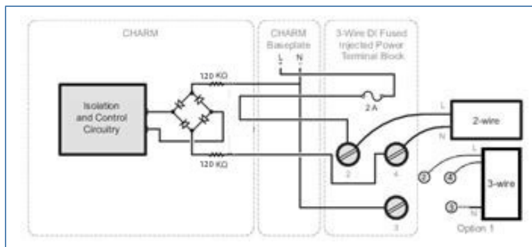
Simplified Circuit and Connection Diagrams for DI 230V AC Isolated CHARM with 3-wire DI Fused-Injected-Power Terminal Block.
