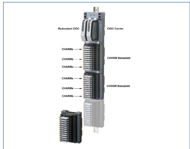
The DeltaV™ CHARM I/O Card (CIOC) with CHARMs.
