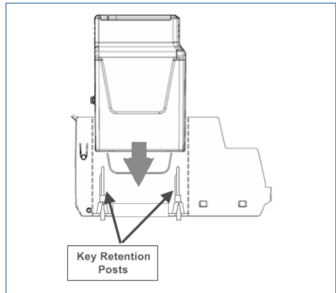
CHARM Standard Terminal block.
