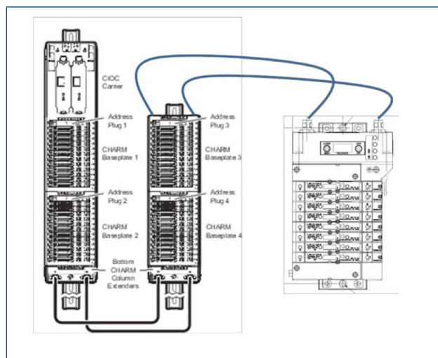
Connection to DeltaV Electronic Marshalling.
