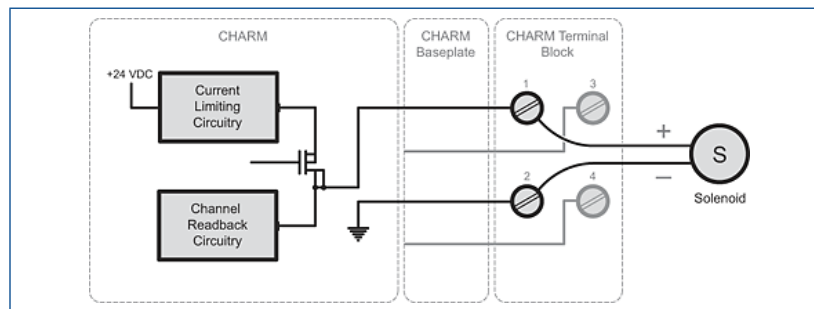
Simplified Circuit and Connection Diagram for DO 24V DC High Side CHARM.
