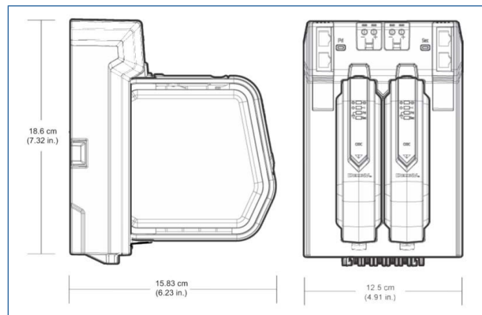
CHARM I/O Card and Carrier.
