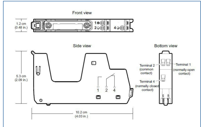
CHARM Relay Output Terminal Block.
