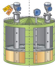
FMCW Radar (5900S) (Pipe)
