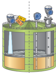
FMCW Radar (5900S) (Roof Plate)
