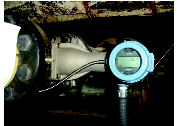
WE Energies' Rosemount 8800 MultiVariable steam installation.
