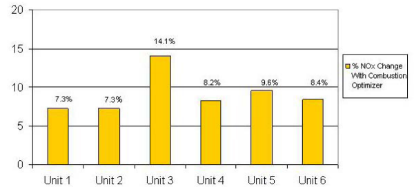
Average percentage of NOx improvement for each Joppa unit.
