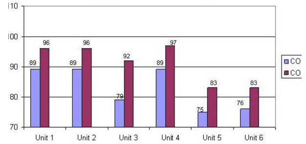
Average NOx readings for each unit with and without the Ovation combustion optimization application.
