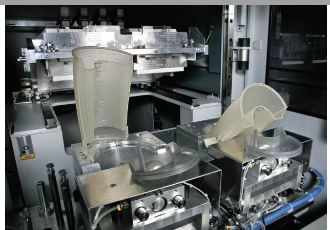
Water reservoir for home appliance.
